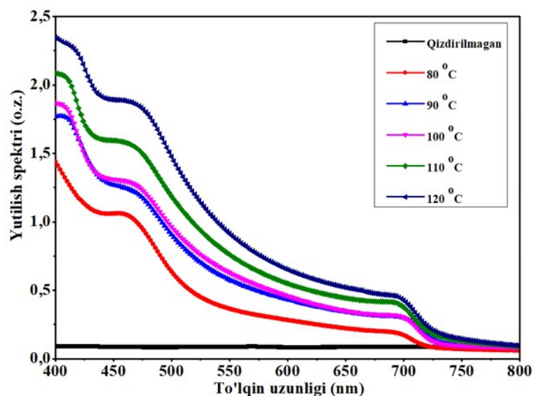
Figure 3. Absorption spectra of CsPbI 3 perovskite active layers prepared using MAAC solvent and thermally heated at different temperatures.
