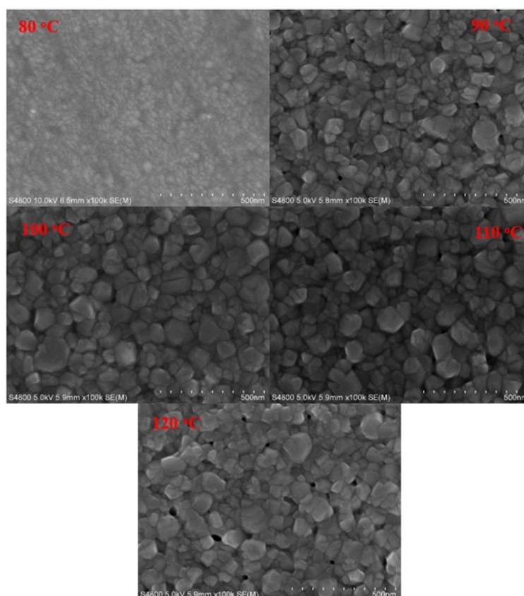
Figure 5. SEM images of perovskite active layers prepared in DMF solvent and heated at different temperatures.
