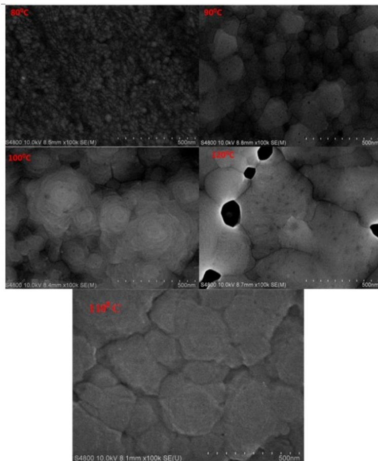
Figure 6. SEM images of perovskite active layers prepared in MAAC solvent and heated at different temperatures.
