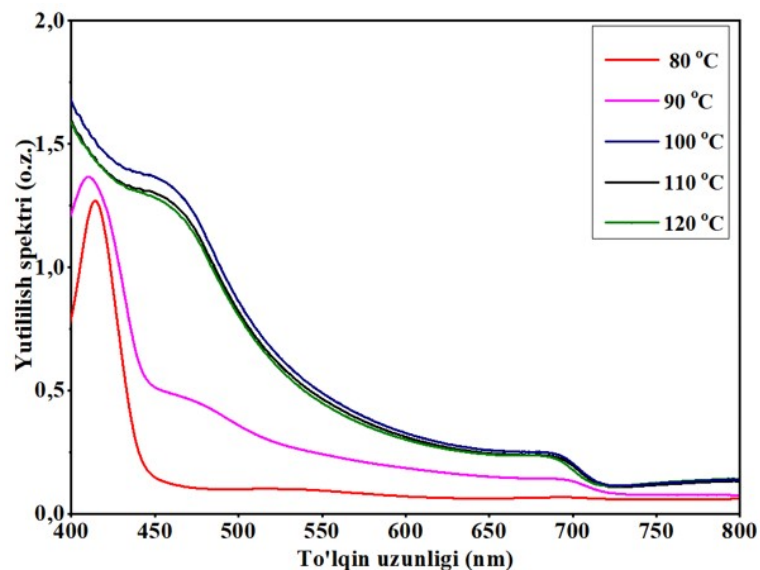
Figure 2. Absorption spectra of perovskite active layers prepared from a perovskite solution in DMF solvent after thermal heating at different temperatures.
