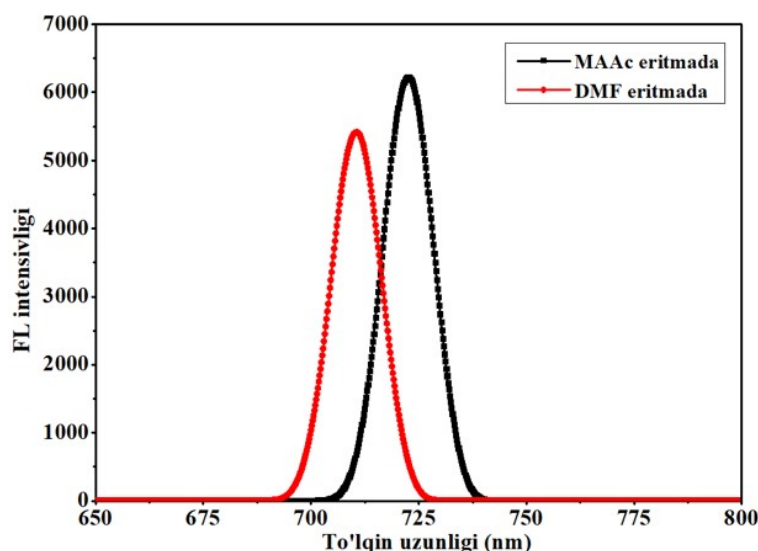
Figure 4. PL spectra of perovskite active layers prepared in MAAC and DMF solvents.
