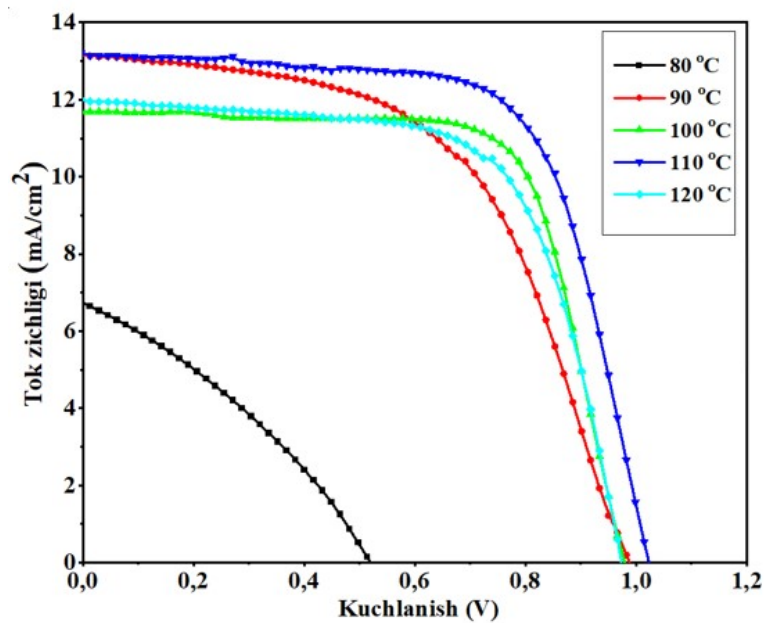
Figure 8. Current-voltage characteristic graph of CsPbI 3 PSCs prepared in MAAC solvent at different heating temperatures.
