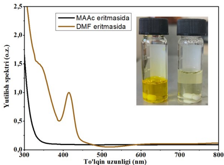
Figure 1. Absorption spectra of CsPbI 3 perovskite active layers prepared in DMF and MAAC solvents before heating.
