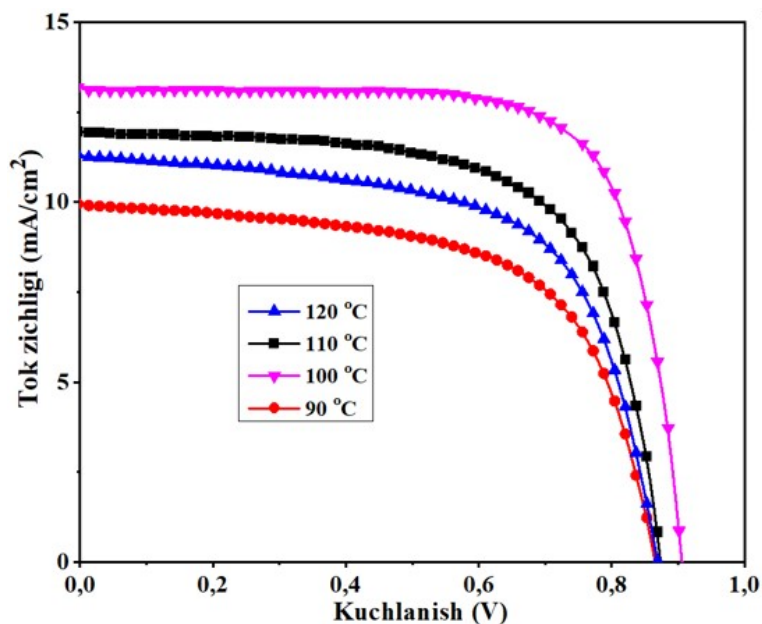
Figure 7. Current-voltage characteristic graph of CsPbI 3 PSCs prepared in DMF solvent at different heating temperatures.
