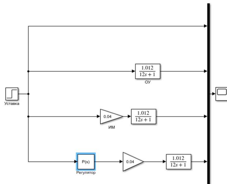
Figure 5. Perfected scheme.
