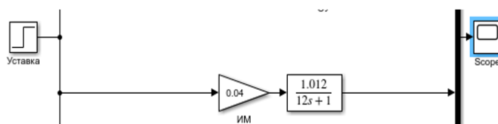
Figure 3. Initial scheme.
