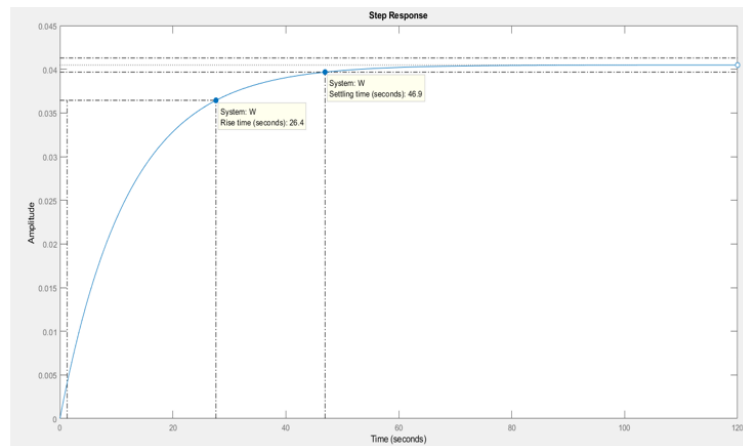
Figure 7. Step Response.
