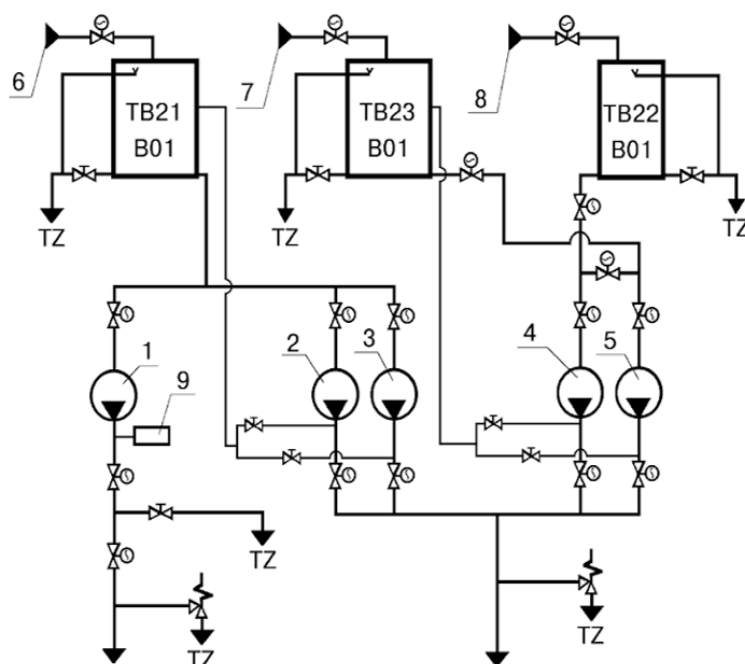
Figure 1. Simplified diagram of the reagent addition system.
