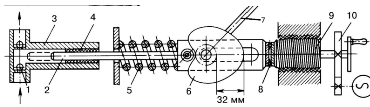
Figure 2. Pump dosing work scheme.
